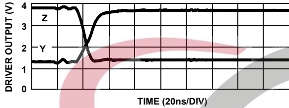
FIGURE 16. DRIVER AND RECEIVER WAVEFORMS, LOW TO HIGH (ISL8490E/ISL8491E)
